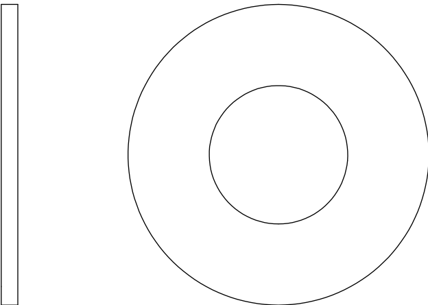
C9. Washer (Ø26.7XØ58X3.2T) Qty.2
