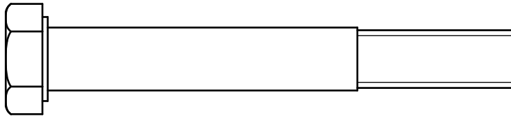
(AA3)HEX BOLT M12X90L PARTIAL THREAD QTY.2
