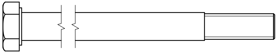
(A1)HEX BOLT M12X140L PARTIAL THREAD QTY.2
