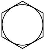
(A2)HEX BOLT M12X60L PARTIAL THREAD QTY.1
