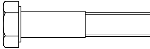
(A2)HEX BOLT M12X60L PARTIAL THREAD QTY.1
